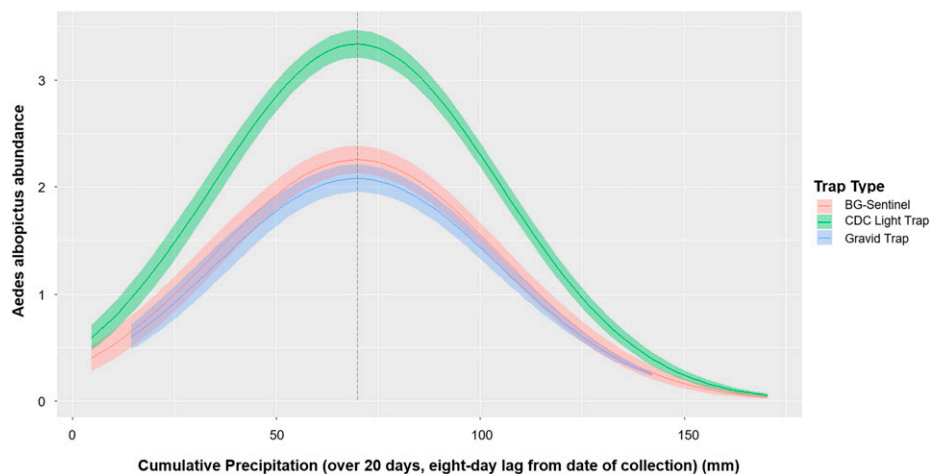
FIGURE 4. Predicted Aedes albopictus abundance as a function of lagged precipitation. Predicted Ae. albopictus abundance as a function of the cumulative precipitation over 20 days, with an eight-day lag from the date of collection (Figure 3), based on Model 4. All predictor variables for Model 4 were held at their mean values and the duration of trapping was assumed to be 24-hours, while we allowed cumulative precipitation to vary over its range. We found a quadratic relationship, with precipitation greater than 68.18 mm associated with decreased Ae. albopictus abundance. This figure appears in color at www.ajtmh.org .
